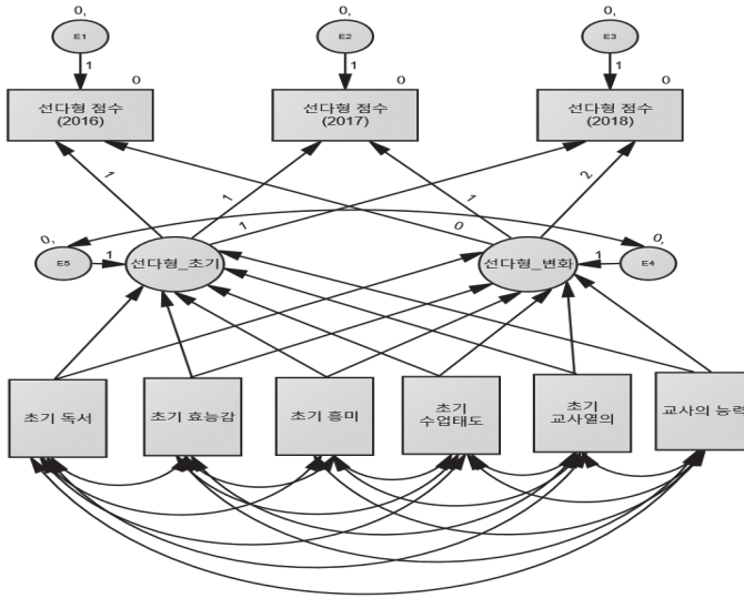
Figure 2. Research model
